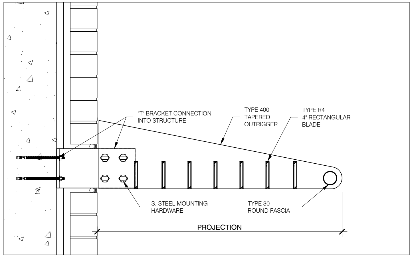
MODEL R4-400-30 CROSS SECTION
