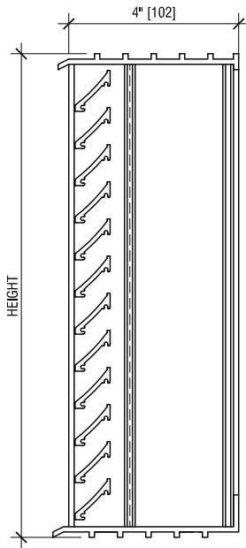
VERTICAL SECTION
